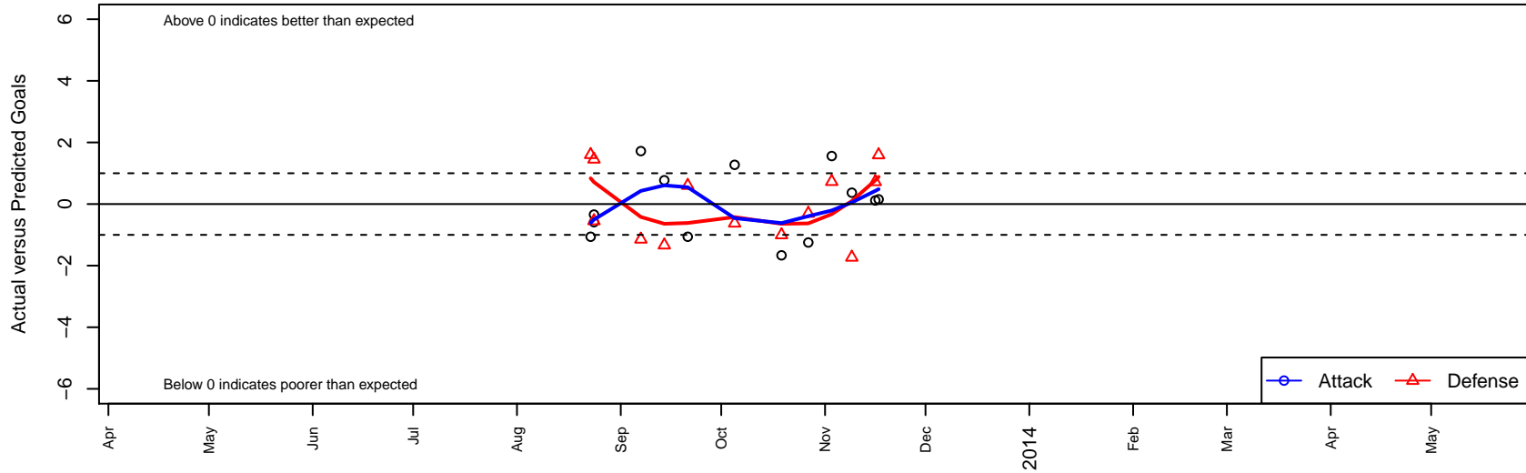
Bay Oaks SC United B00 Dots are actual minus expected GF (blue circles) and GA (red triangles). Blue line is smoothed change in attack strength. Red is smoothed change in defense strength.
